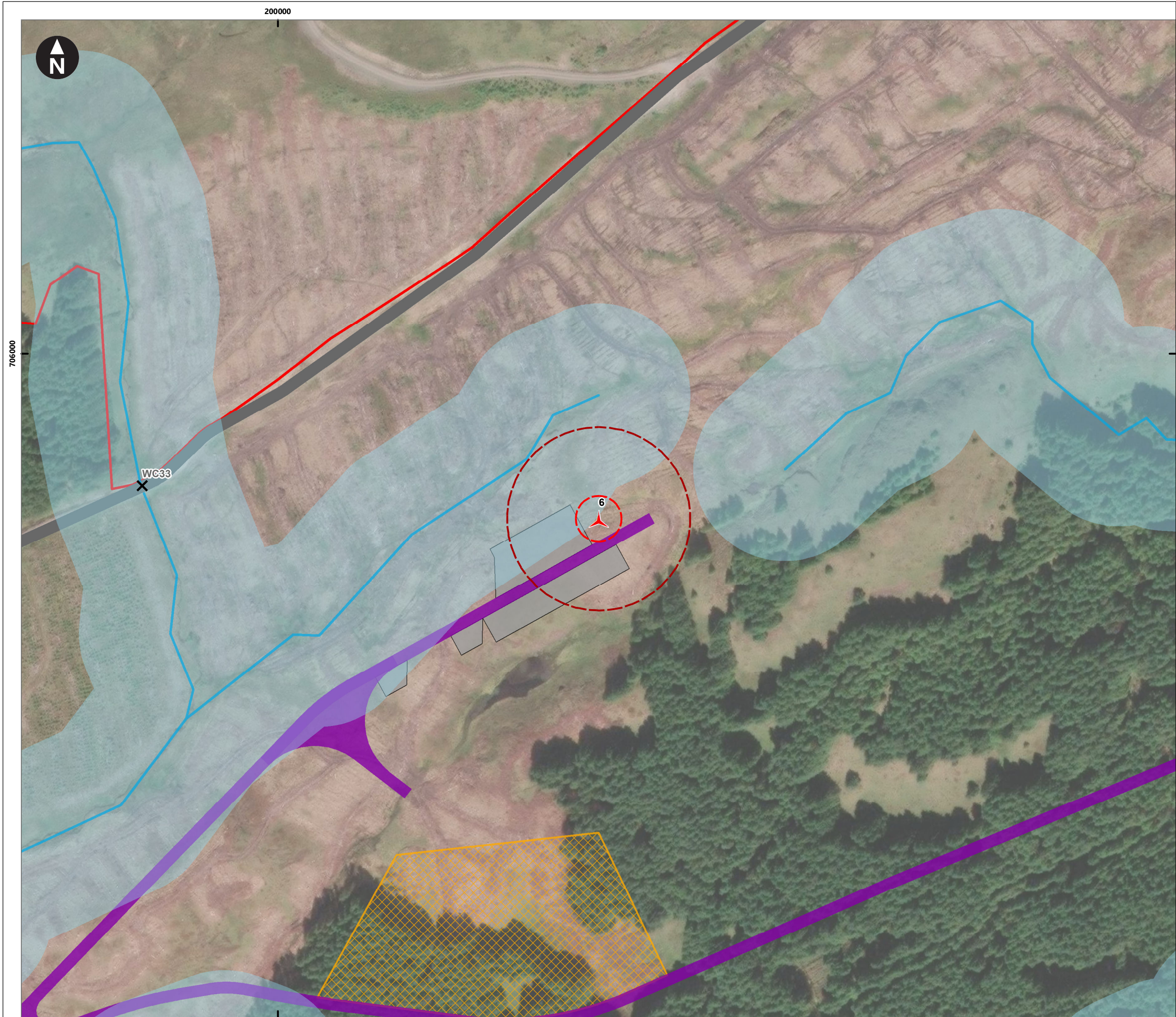
Figure 3.2b Detailed Aerial Imagery of Turbine 6
